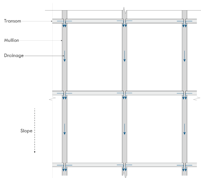
Skylight glazing system: Plan view of the secondary drainage Figure 1
