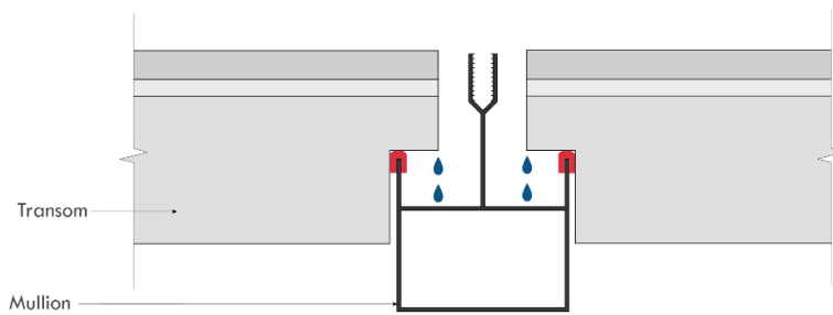
Skylight glazing system: Section - mullion/transom assembly Figure 2
